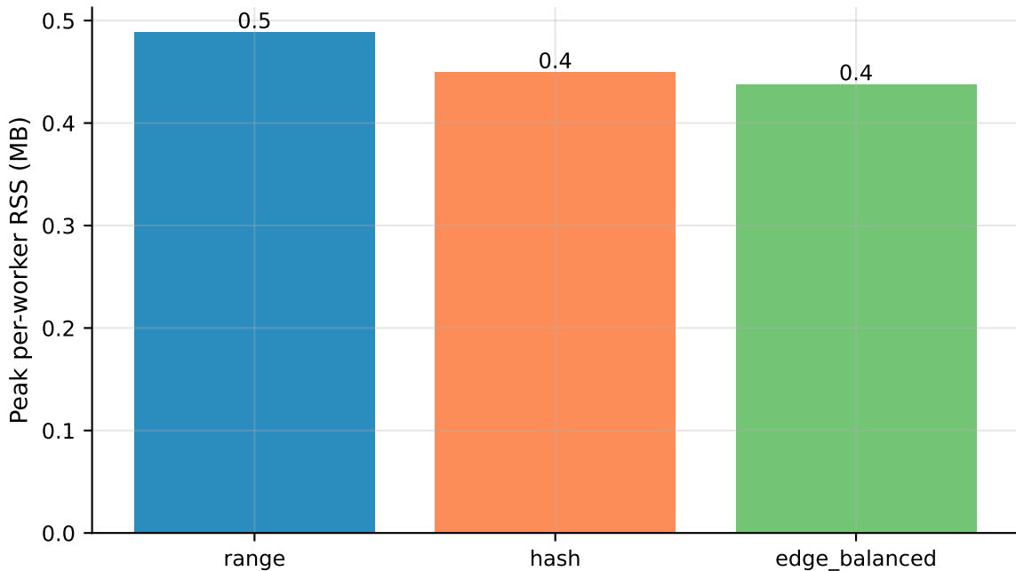
Group B - Peak memory per worker
